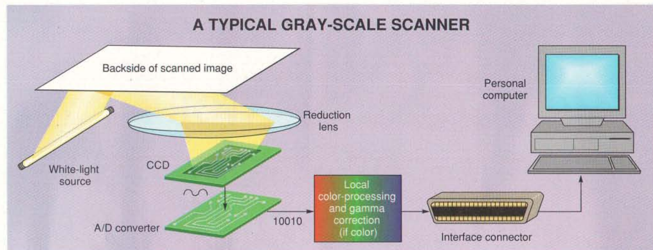
Figure 1: A reduction lens focuses white light reflected from the document onto a CCD (charge-coupled device). The CCD's light sensors output voltages to an A/D converter.
